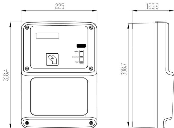
WB Smart series – General dimensions
