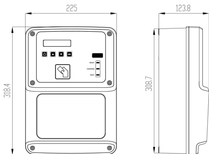
WB Touch series – General dimensions
